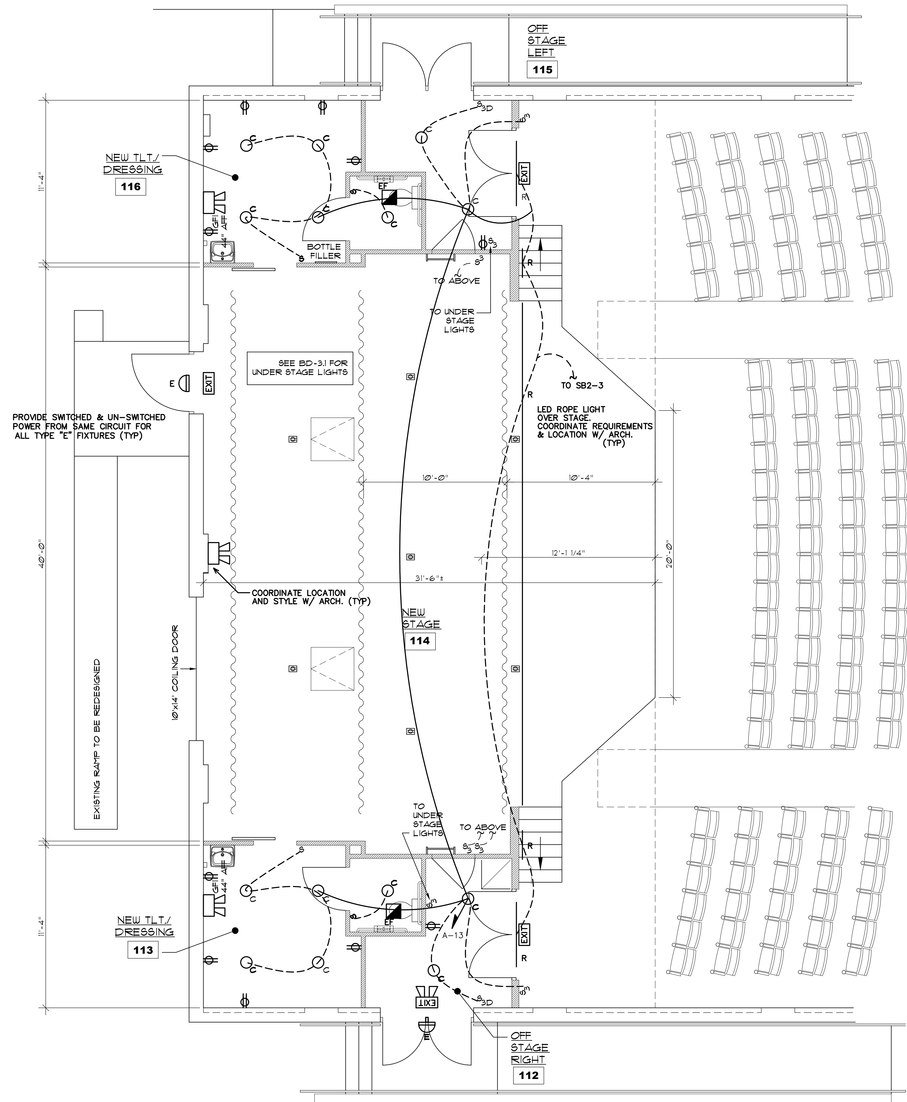
1 REVISED STAGE FIRST FLOOR PARTIAL ELECTRICAL PLAN 5D-32 SCALE: 1/4"=1'-0"
