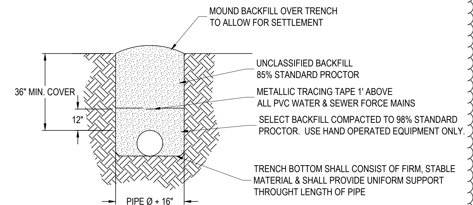
1 PIPE TRENCH OUTSIDE PAVED AREA SCALE: NOT TO SCALE
