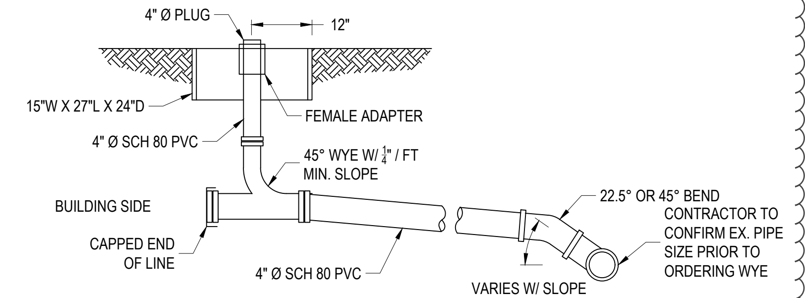
1 SANITARY SEWER CLEANOUT SCALE: NOT TO SCALE
